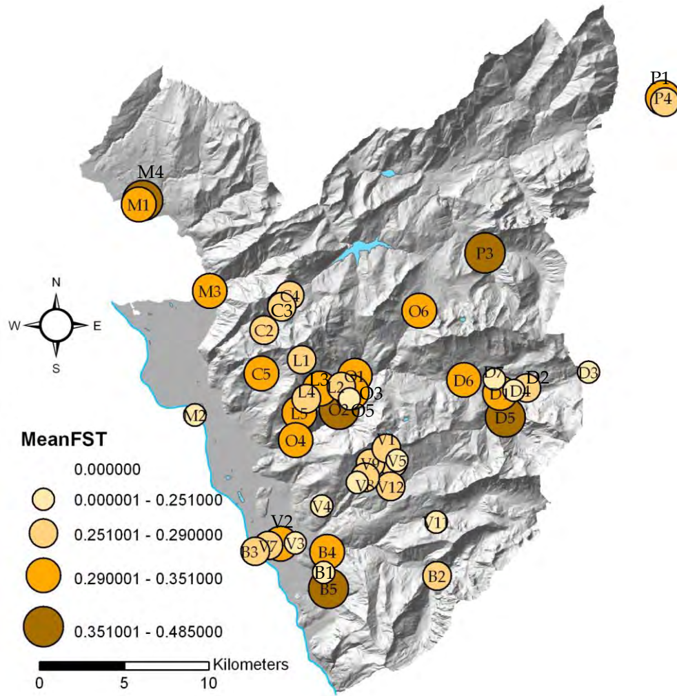
Figure 6. Mean values of pairwise F_{ST} . Sampling locations are indicated by circles of width corresponding to their mean pairwise F_{ST} values. (D-Diablerets, L-Leysin, O-Ormont-dessous, V-Villars, C-Corbeyrier, M-Montreux, P-Pays d'enhaut, B-Bex, S-Caucasus).
